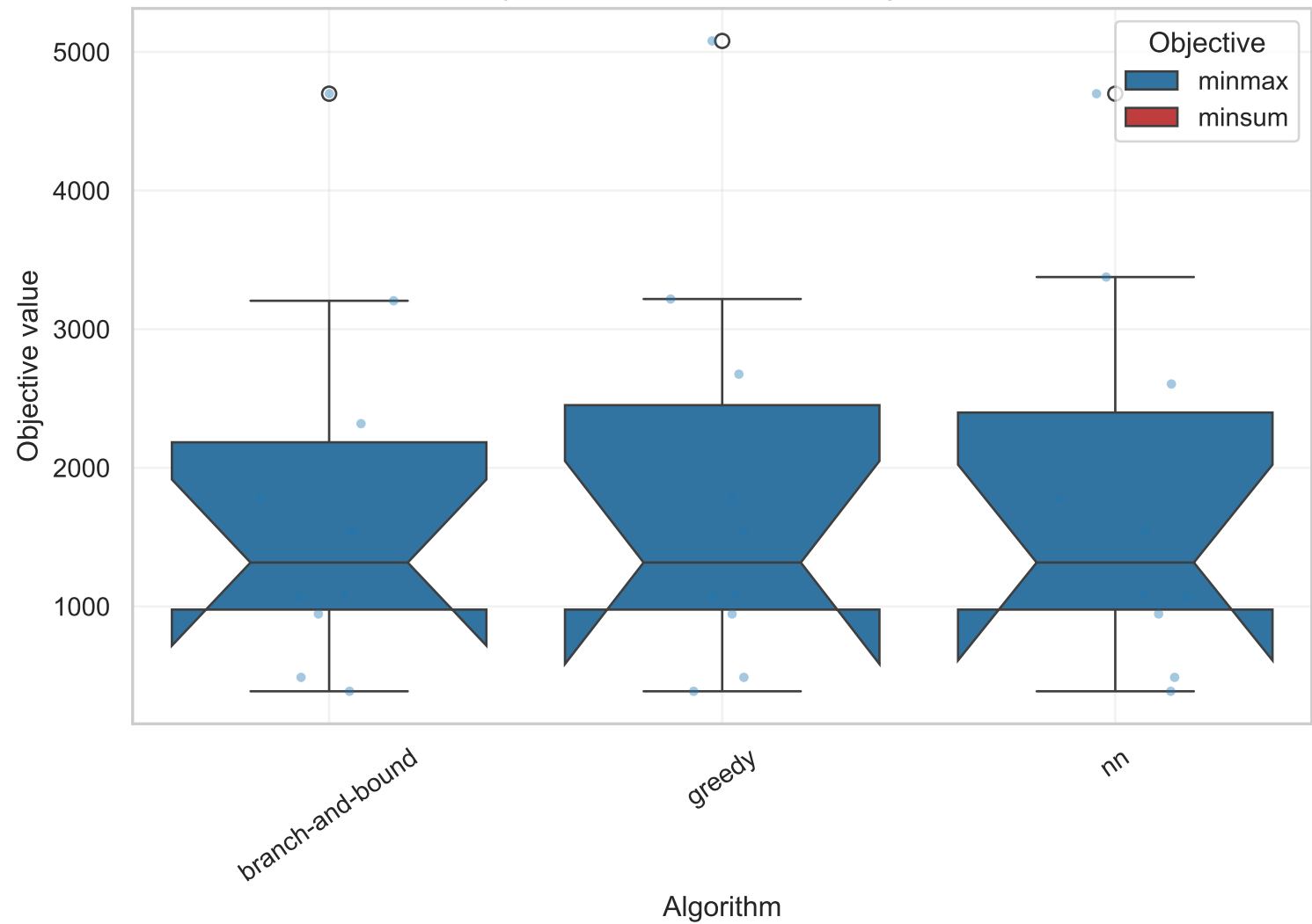
Objective value distribution per algorithm
