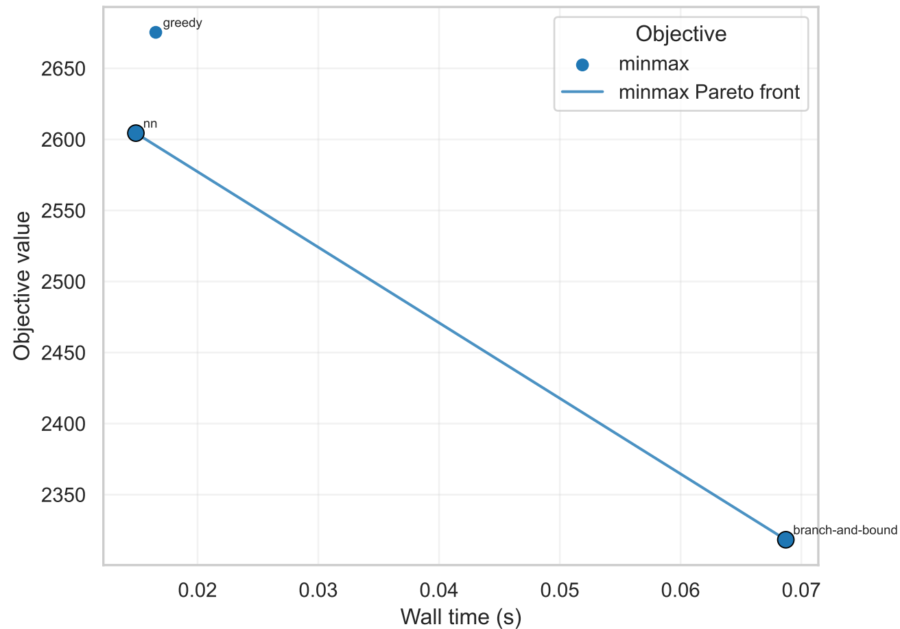
Pareto front on att48
