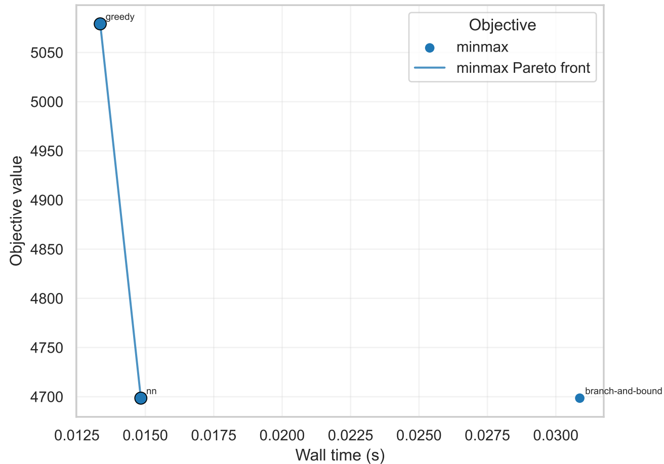
Pareto front on berlin52
