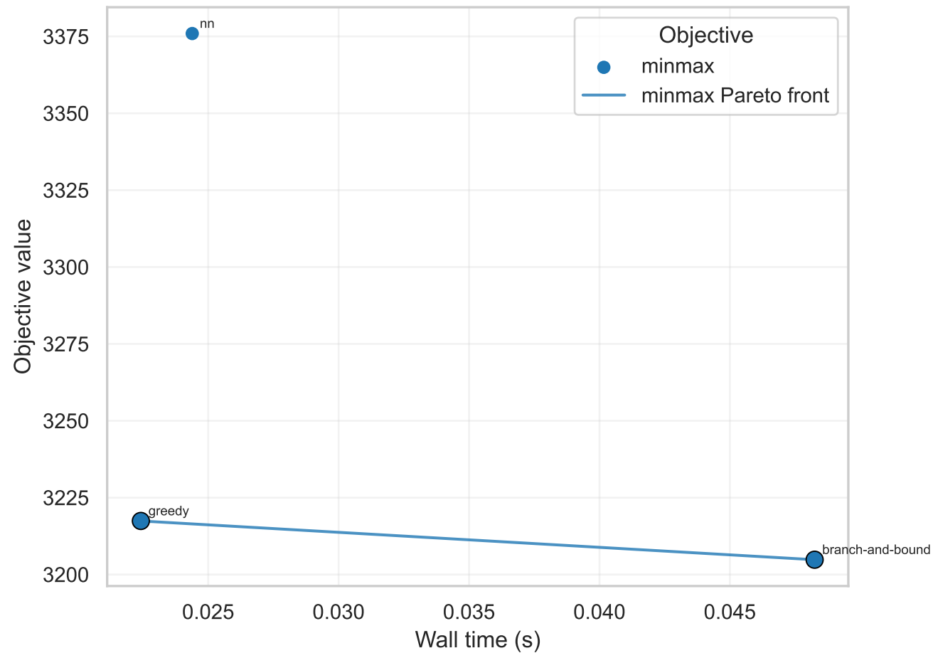
Pareto front on eil51
