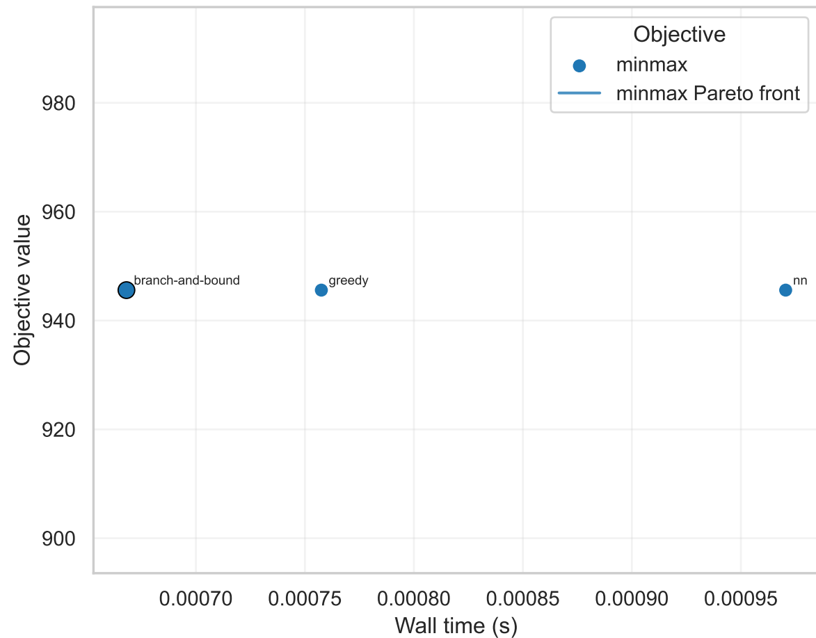
Pareto front on london-0000030.instance
