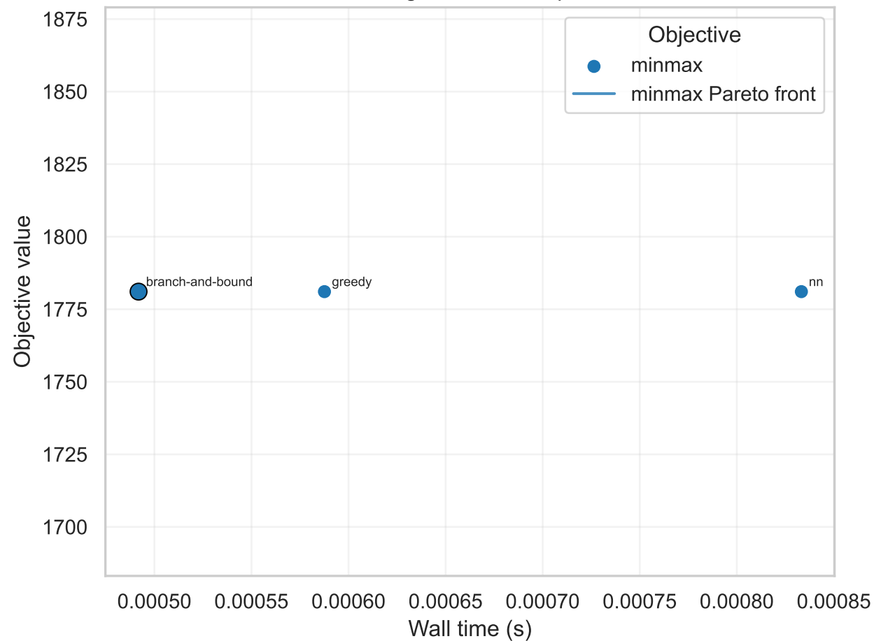
Pareto front on sbgdb-20200507-pntset-0000030
