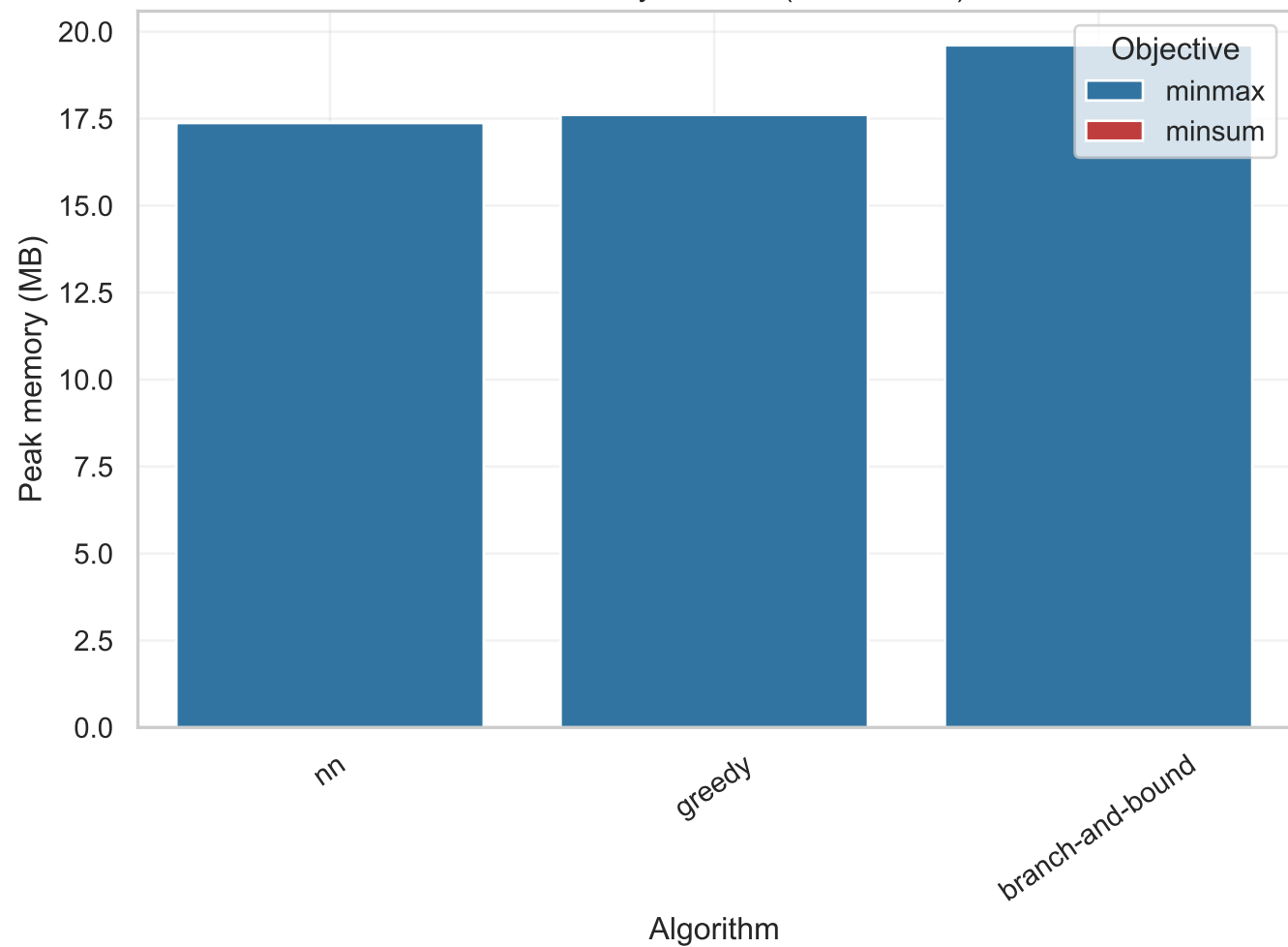
Peak memory on att48 (n=11, m=25)
