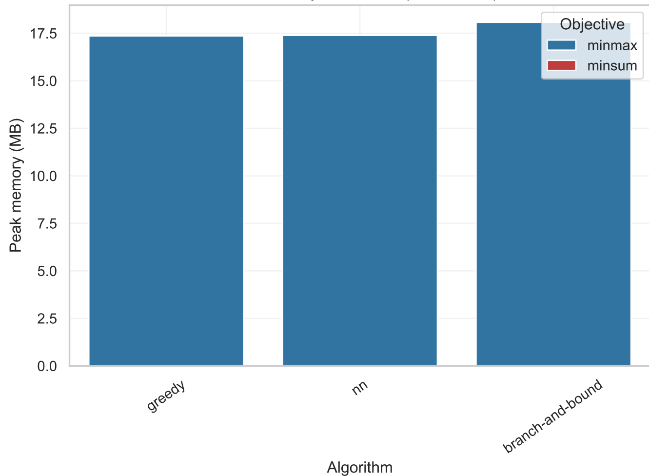
Peak memory on berlin52 (n=13, m=25)
