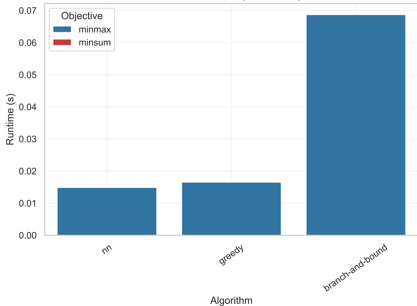
Runtime on att48 (n=11, m=25)
