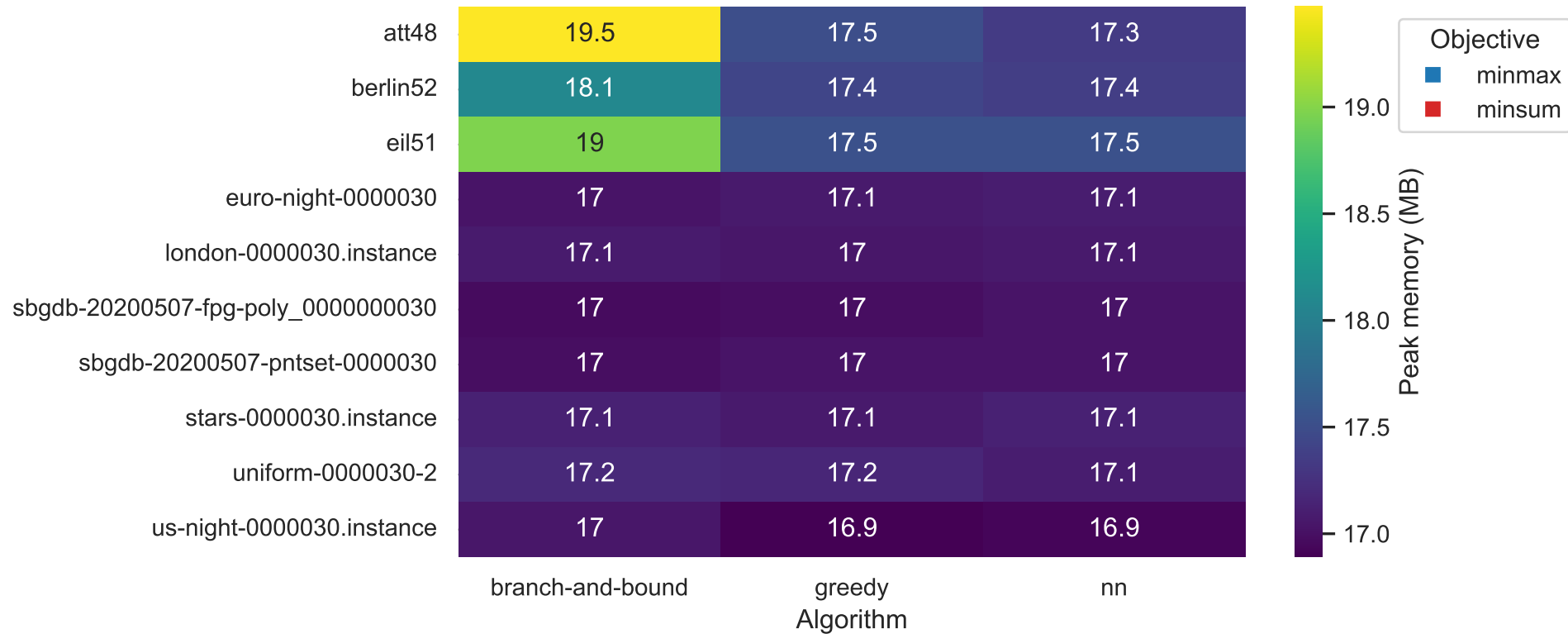
Peak memory heatmap (median across objectives)
