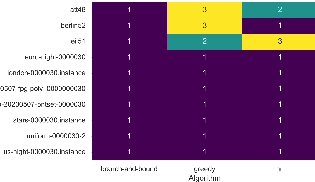
Quality heatmap (rank per instance)
