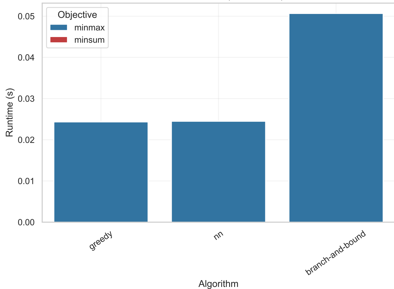
Runtime on eil51 ( n=13 , m=25 )
