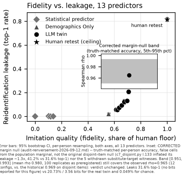
Figure 2: Imitation quality against leakage, with its control. Abscissa: individual fidelity (fidelity_plancher, share of the human floor). Ordinate: closed-world top-1 leakage. Thirteen points – LLM twins, statistical reference points, Demographics Only, and the human retest at fidelity \approx 1 / leakage 81.6 % – all with error bars on both axes from a per-person bootstrap of 2,000 resamples. Inset: the 5th–95th percentile envelope of the corrected marginal null (mean rho 0.980, 100 replicates) as a grey band, with the observed rho (0.965) inside it: the observed correlation sits inside the band that a null matched only on accuracy already produces – the coupling is measured, not shown to be individual-specific.
