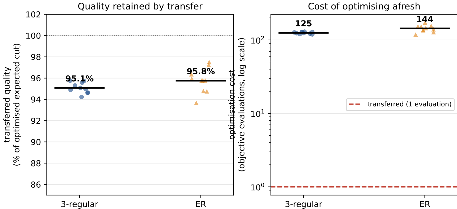
Figure 5.4 — Transfer keeps ~95% of optimised quality at a fraction of the cost
