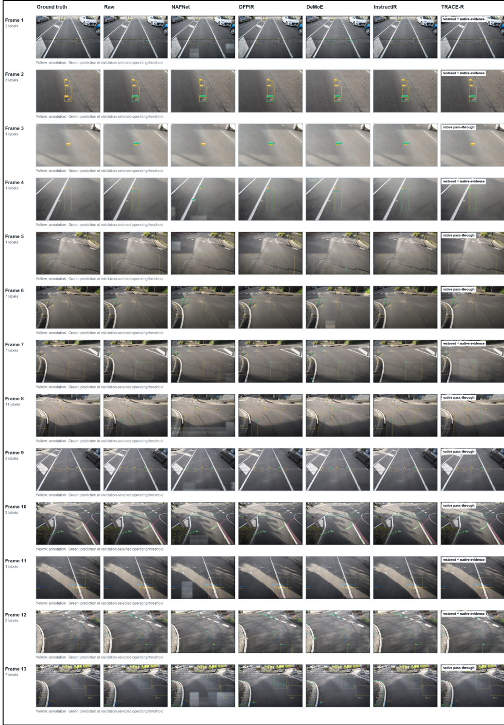
Fig. 3. All 13 CRID temporal-evaluation frames. Yellow boxes are annotations and green boxes are predictions at validation-fixed operating thresholds. TRACE-R labels each frame as native pass-through or native-plus-restored evidence.
