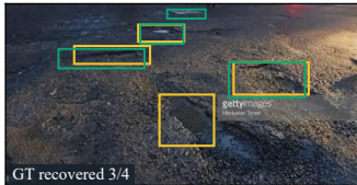
DeMoE
