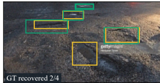
FiLM-NAFNet
