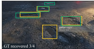
TRACE-R
