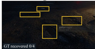
Degraded
