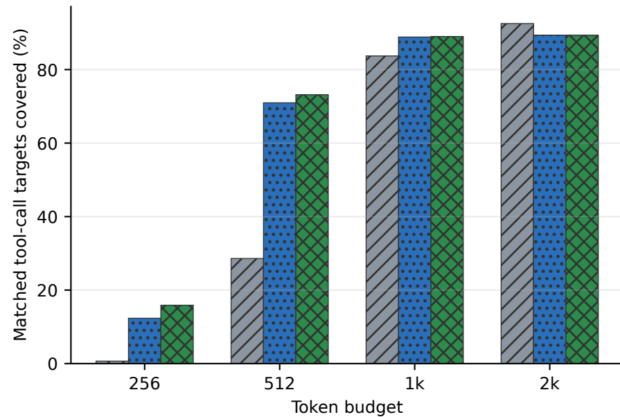
(a) ToolACE
