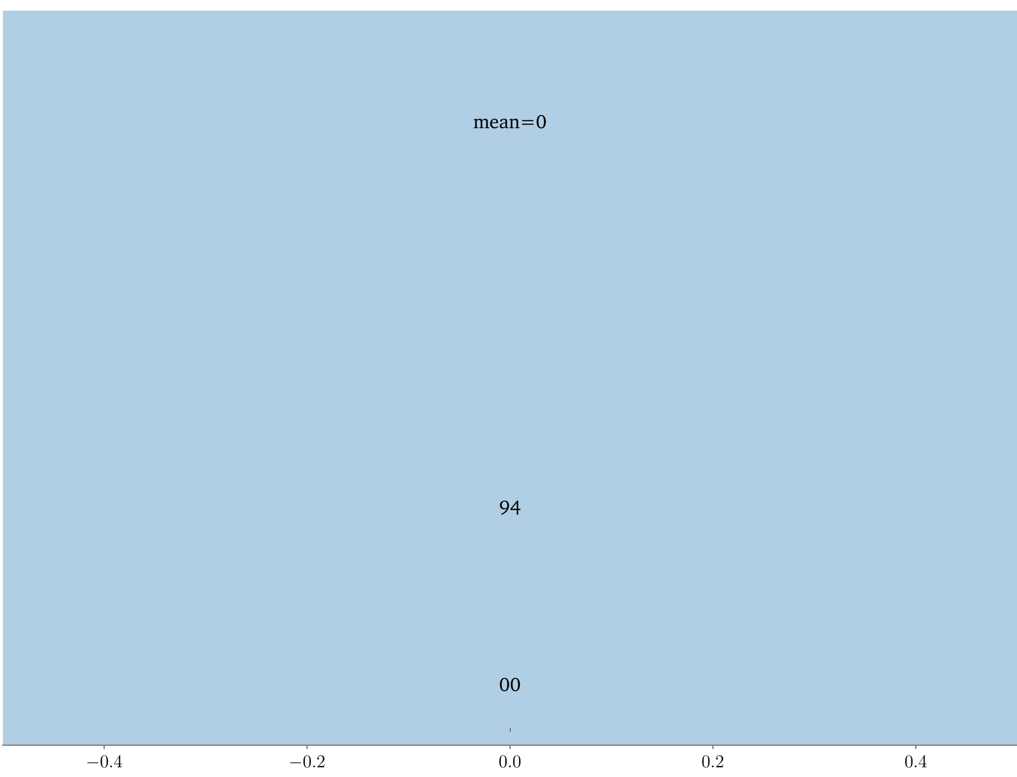
beta_bias_sampler
