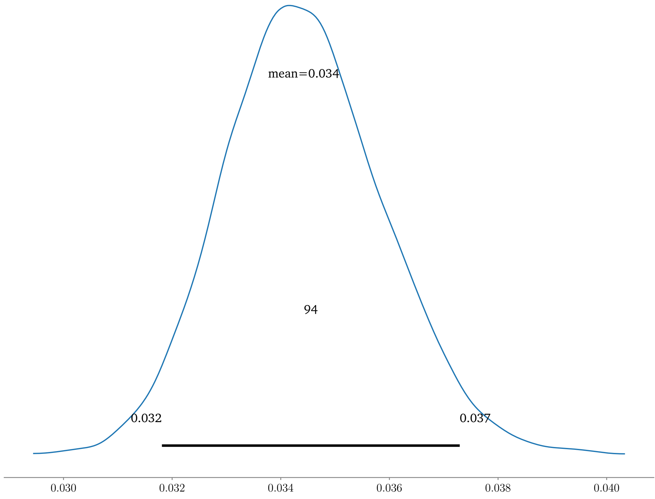
sigma
