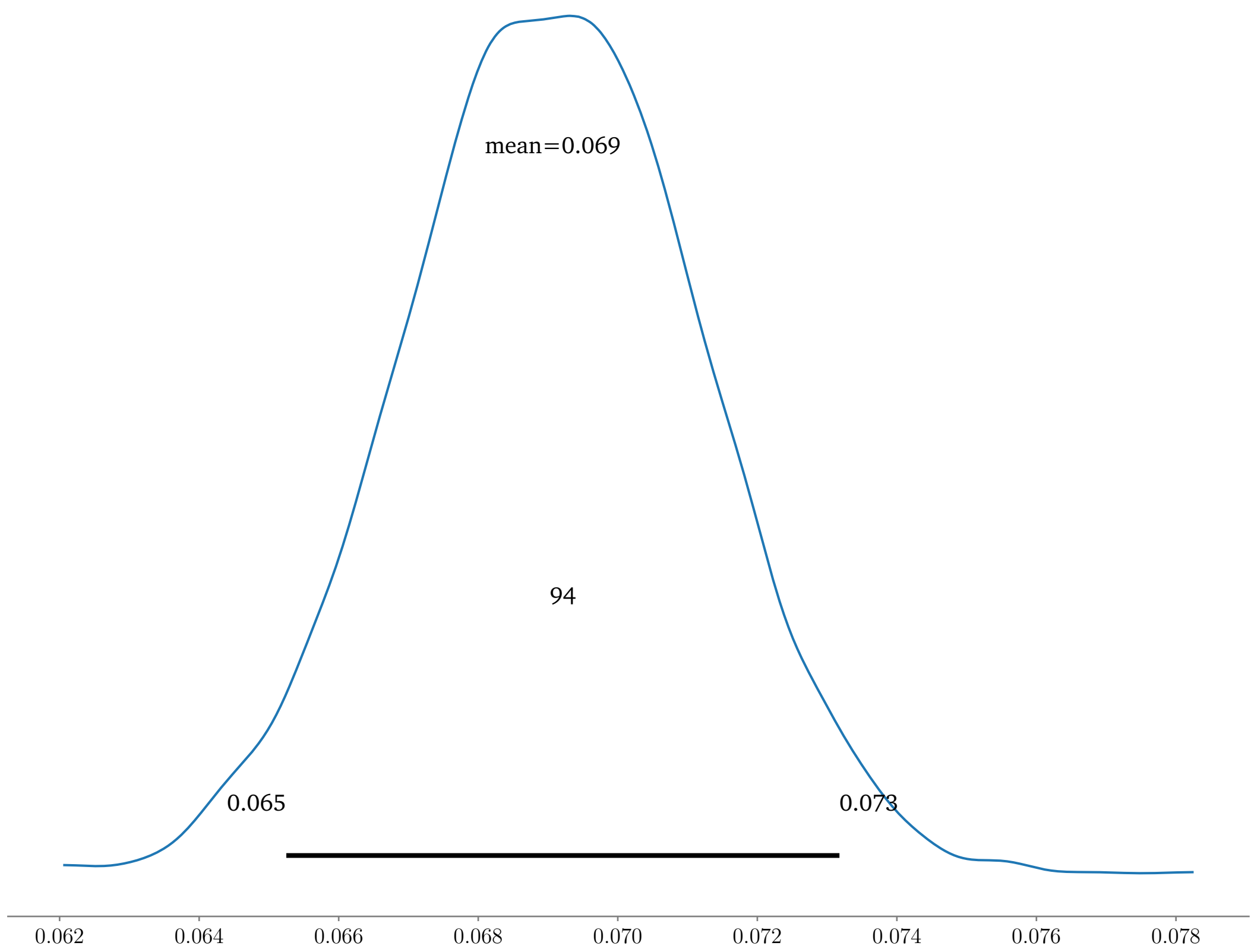
beta_bias.candidates
