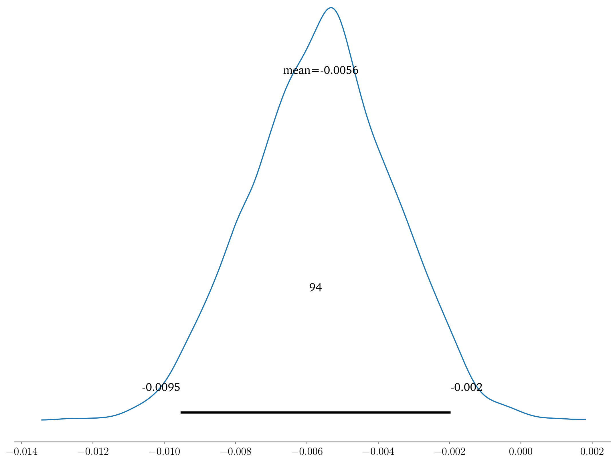
beta_bias.voters
