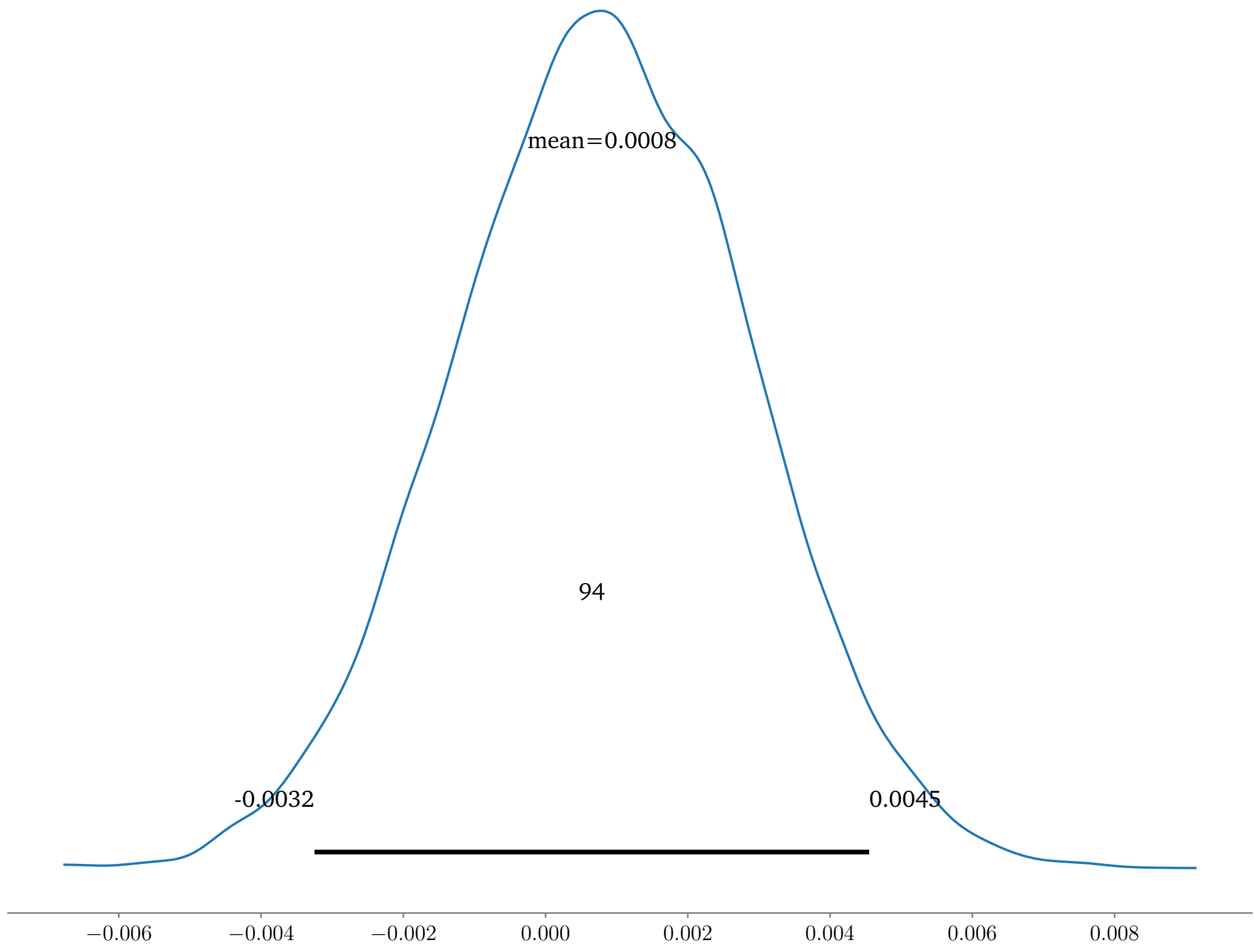
sigma
