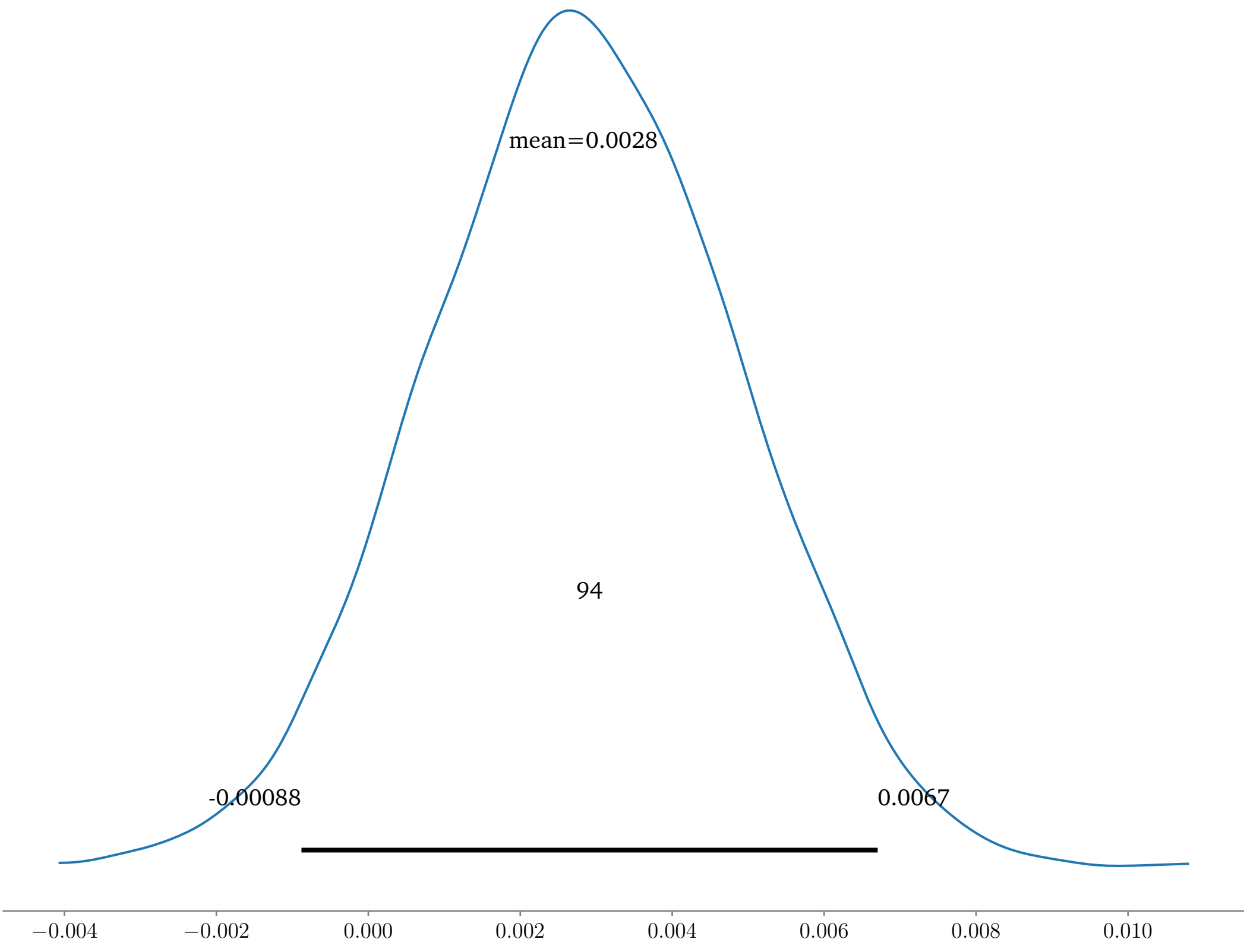
beta_bias_sampler
