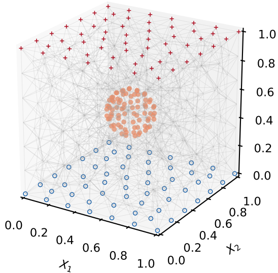
(b) 3D spherical inclusion
