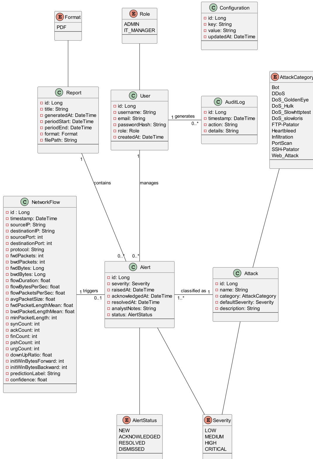
FIGURE 3.1 – Class Diagram
