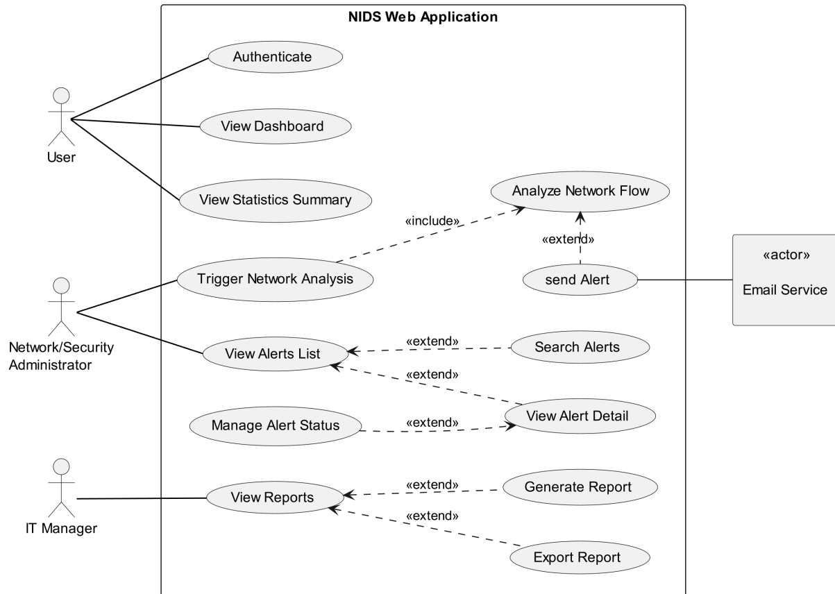
FIGURE 2.2 – Use Case Diagram
