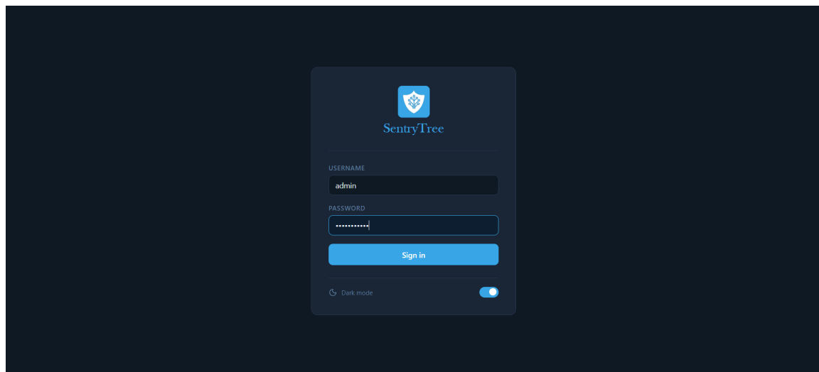
FIGURE 6.5 – Authentication interface
