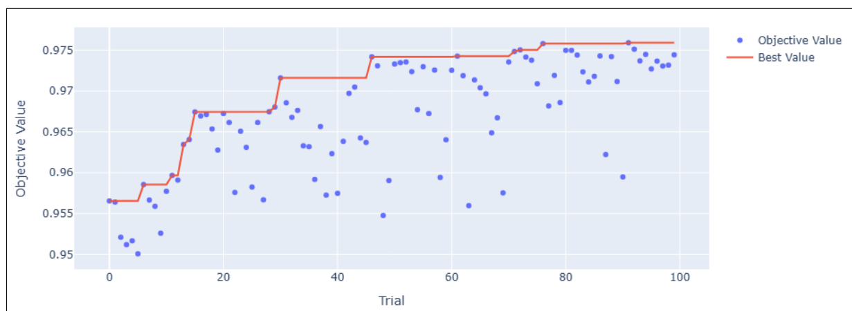
FIGURE 5.5 – Optimization history
