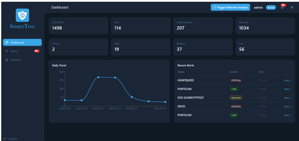
FIGURE 6.6 – Dashboard interface
