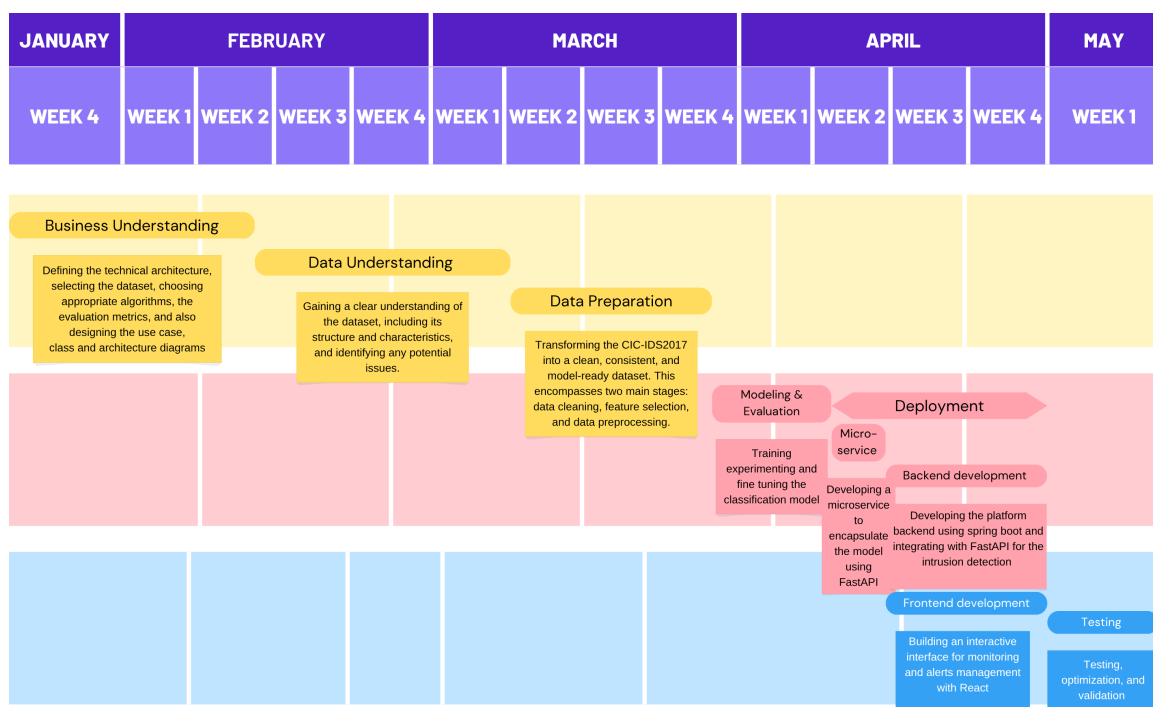
FIGURE 1.1 – Project Pipeline
