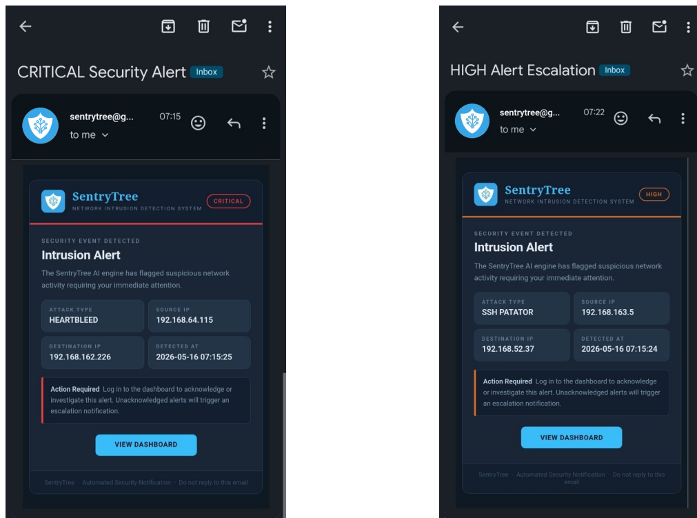
FIGURE 6.11 – Email notifications
