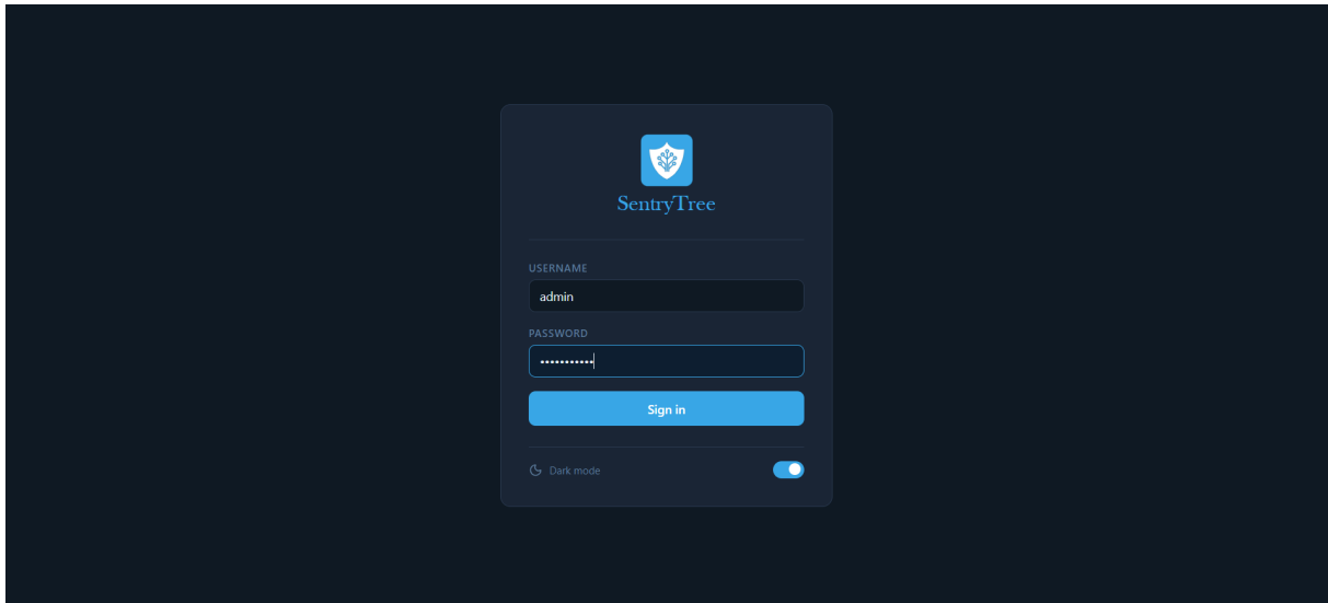
FIGURE 6.5 – Authentication interface
