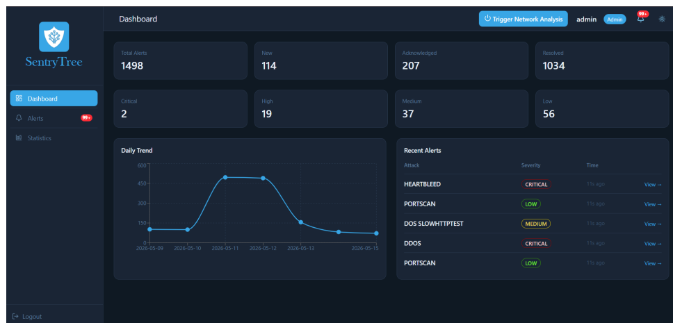
FIGURE 6.6 – Dashboard interface
