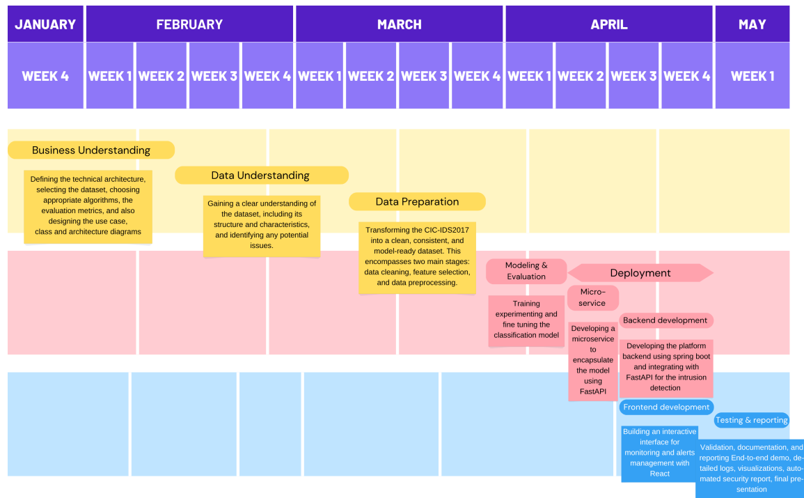
FIGURE 1.1 – Project Pipeline
