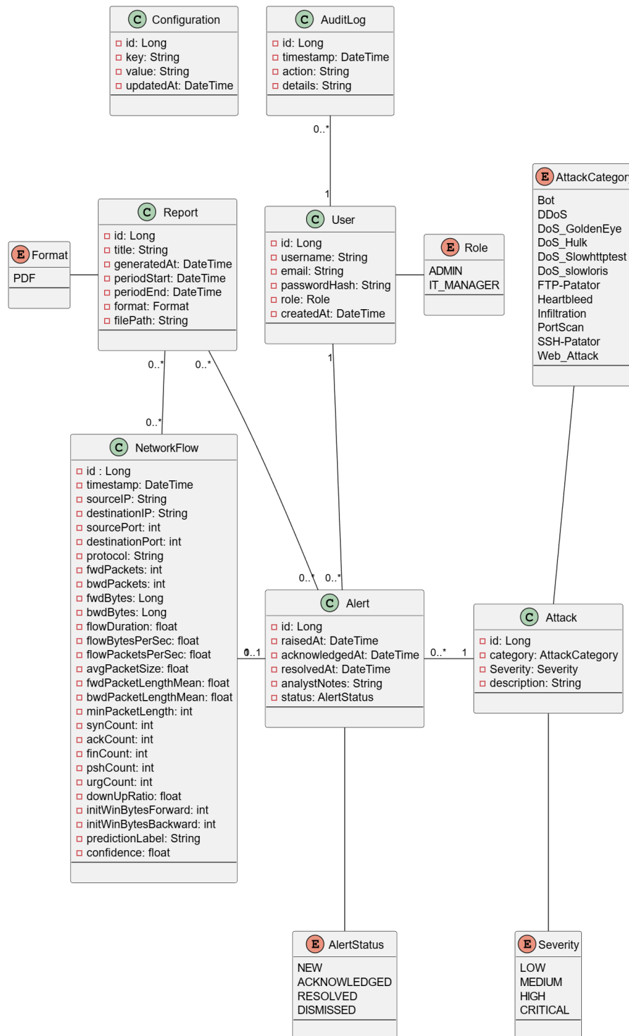
FIGURE 3.3 – Class Diagram
