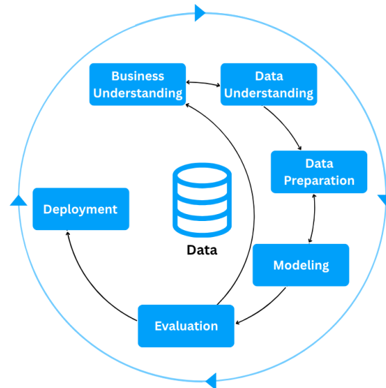
FIGURE 1.2 – CRISP-DM Methodology
