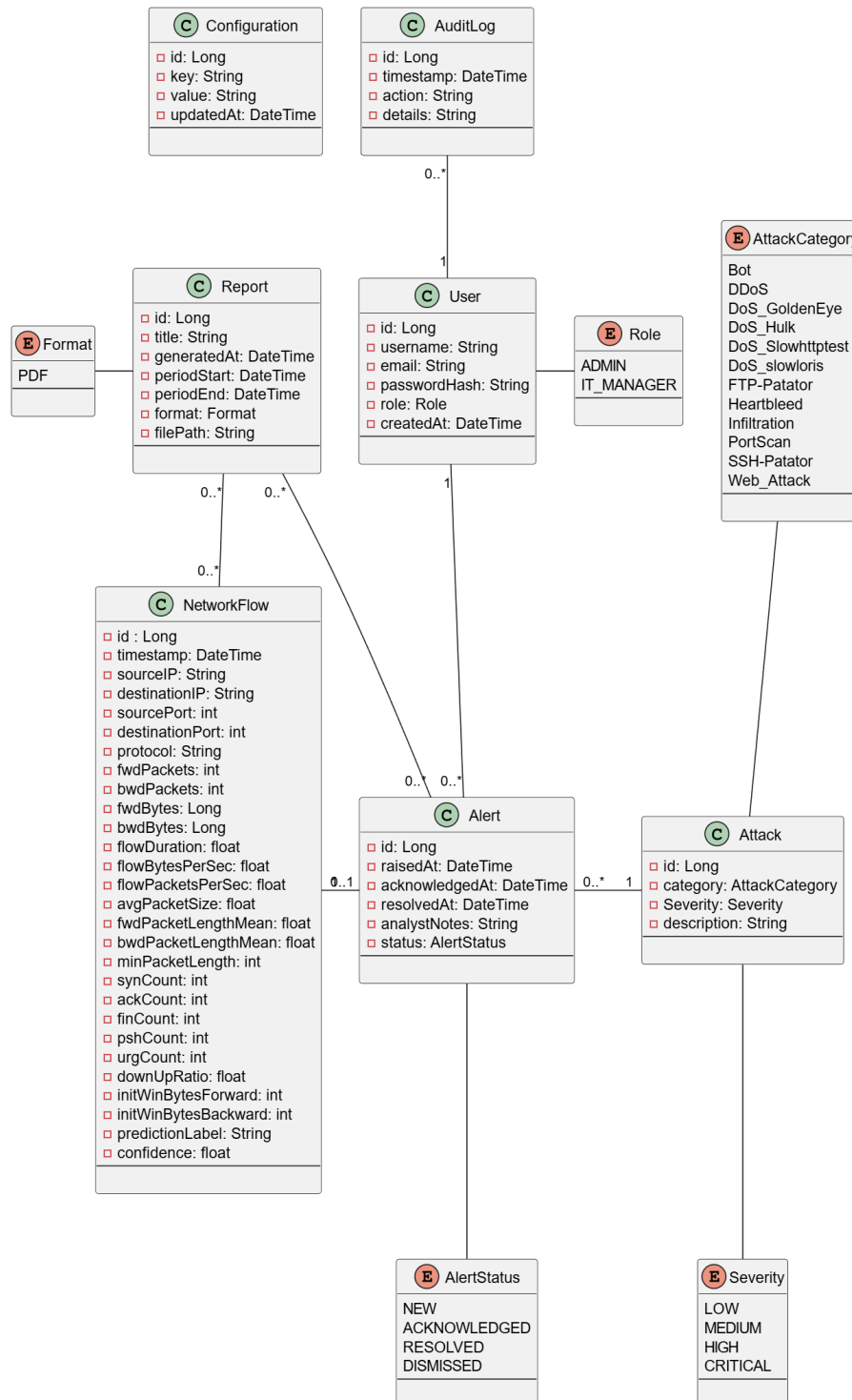
FIGURE 3.3 – Class Diagram
