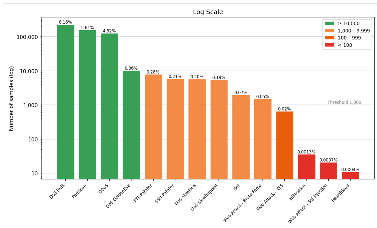
FIGURE 4.5 – Attack distribution
