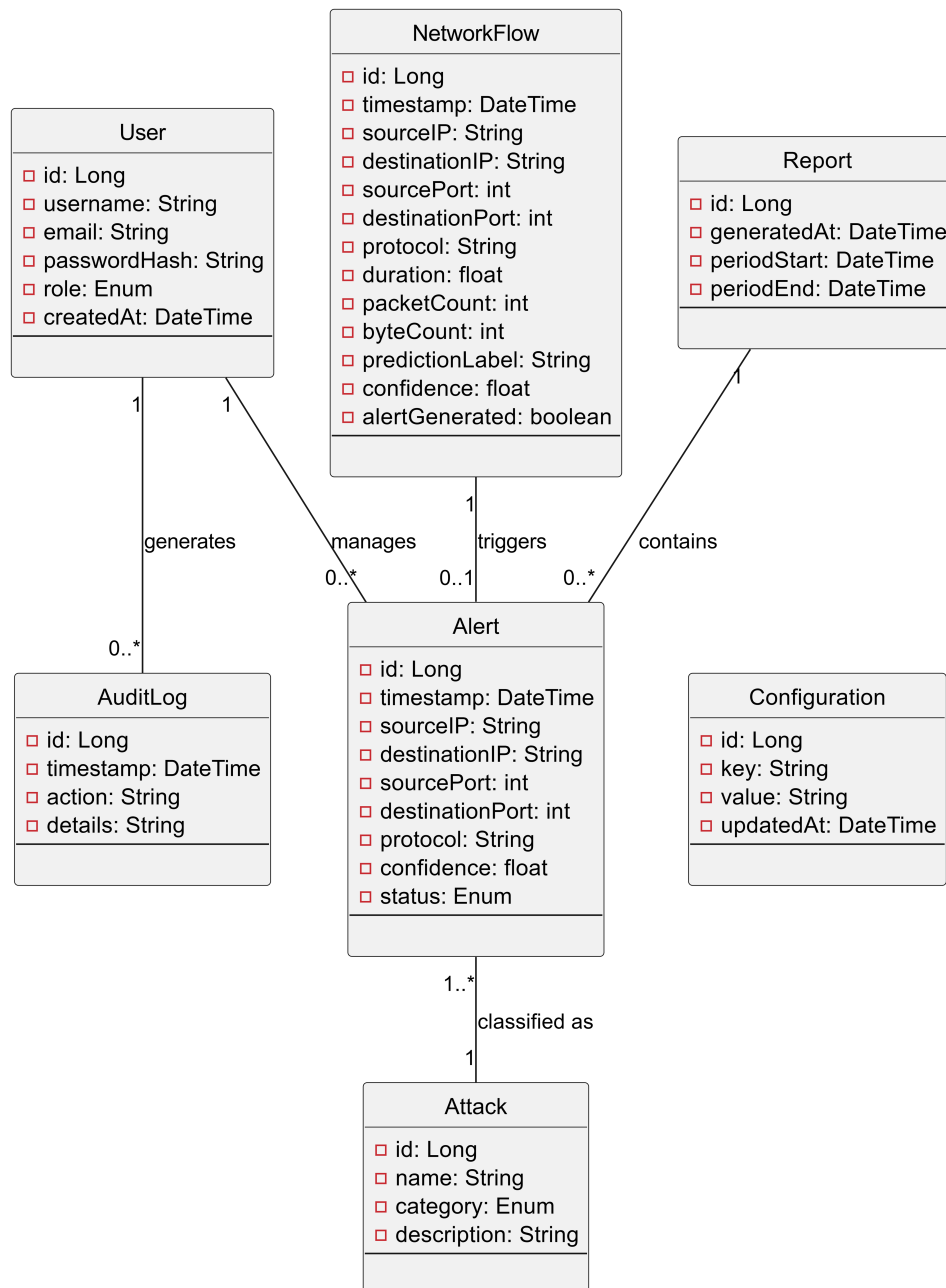
FIGURE 3.1 – Class Diagram
