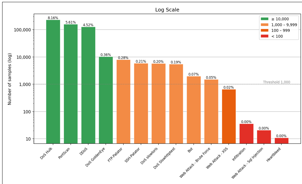
FIGURE 4.5 – Attack distribution
