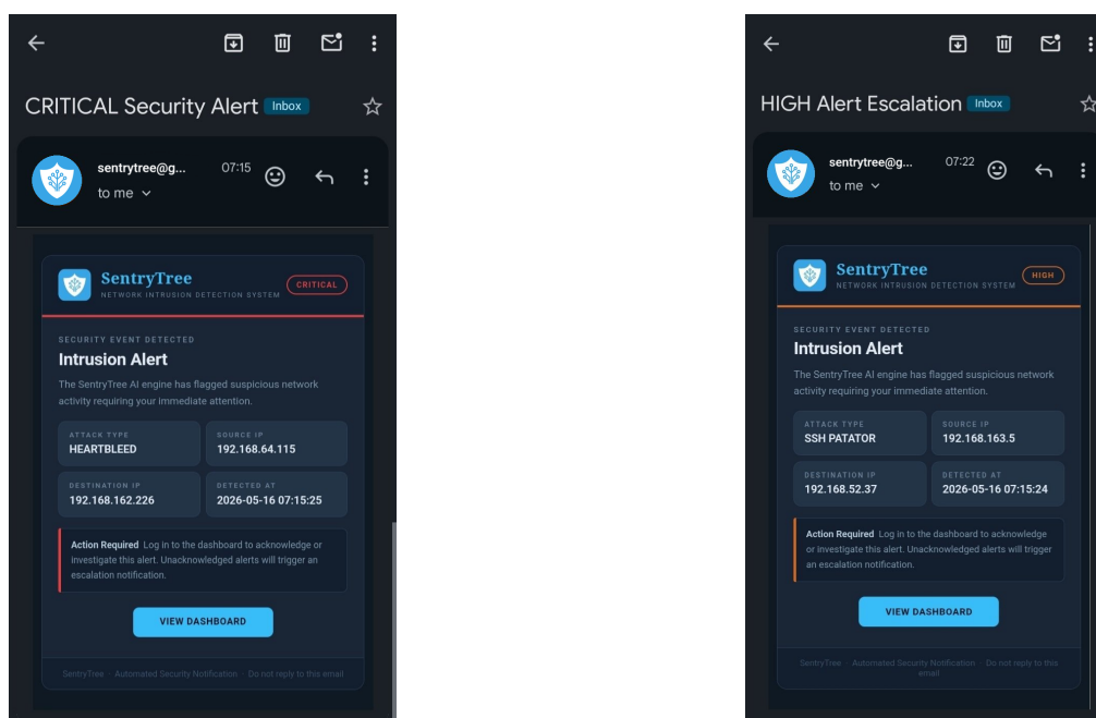
FIGURE 6.11 – Email notifications
