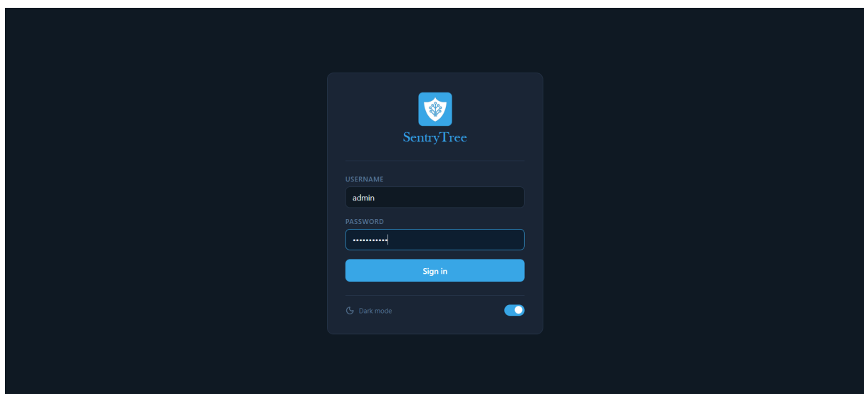
FIGURE 6.5 – Authentication interface
