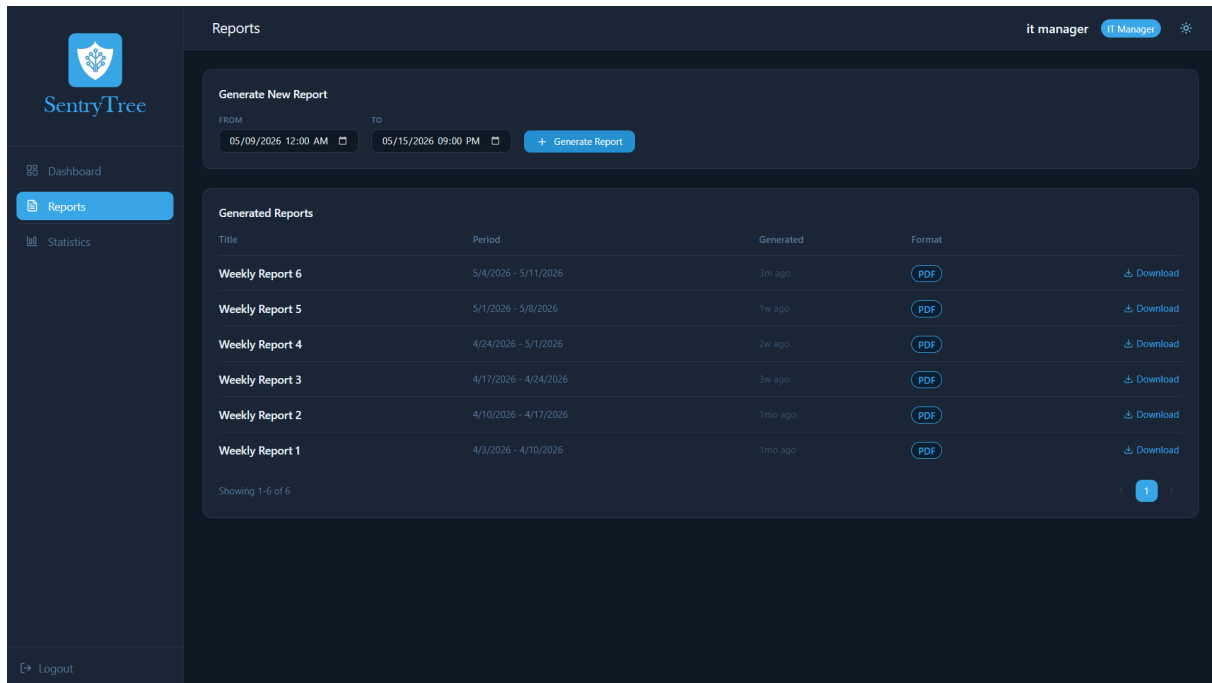
FIGURE 6.16 – Reports interface
