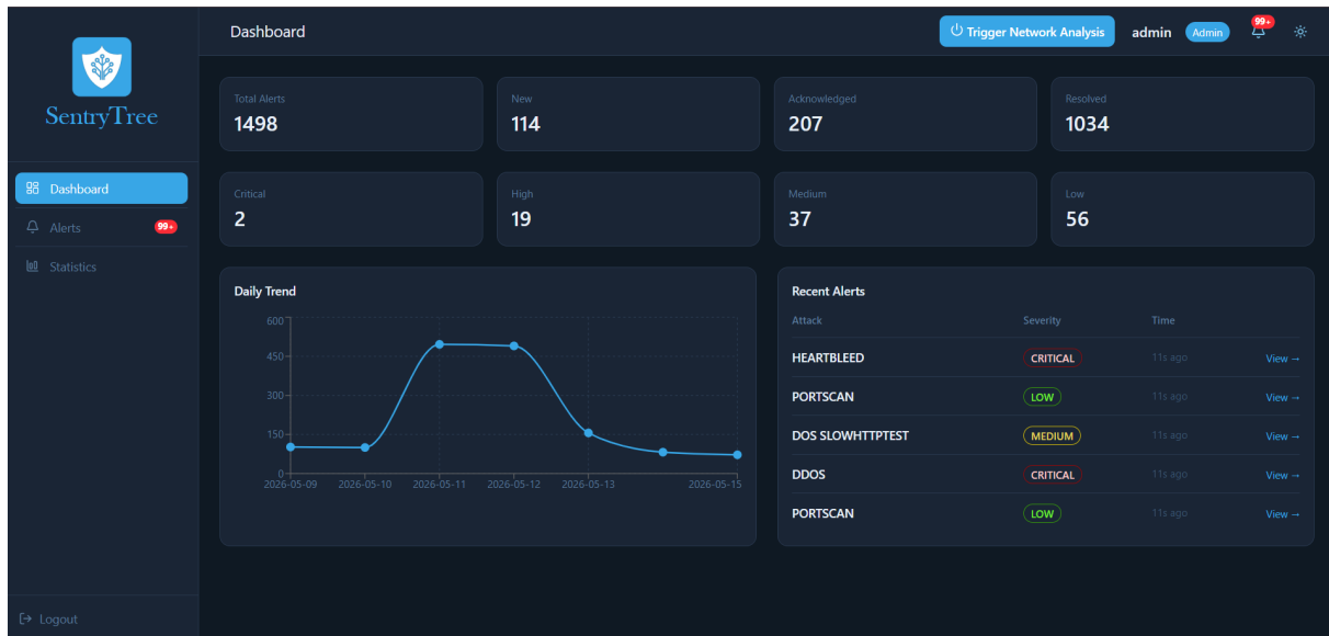
FIGURE 6.6 – Dashboard interface
