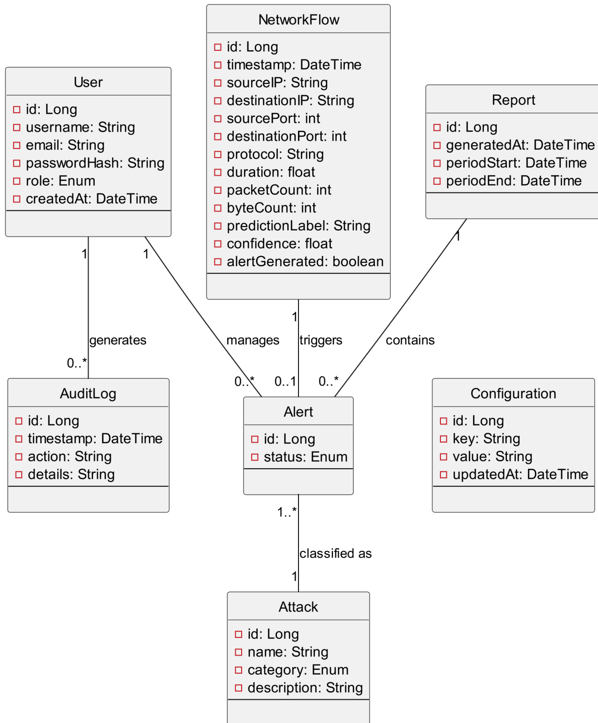
FIGURE 3.1 – Class Diagram
