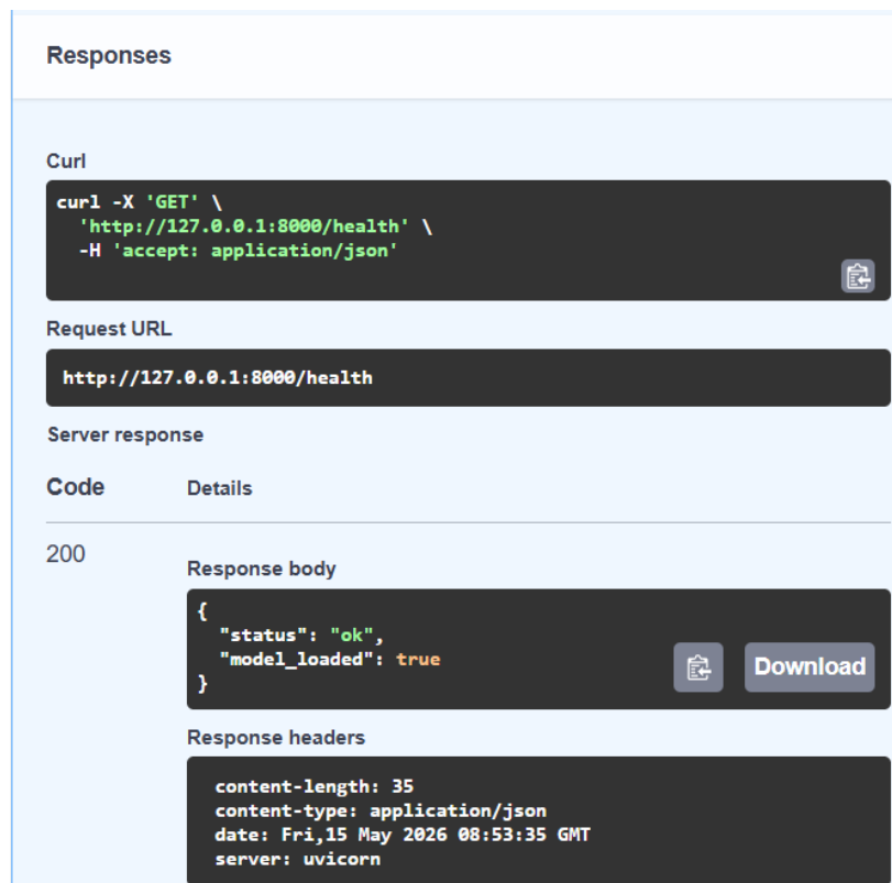
FIGURE 6.1 – FastAPI /health endpoint
