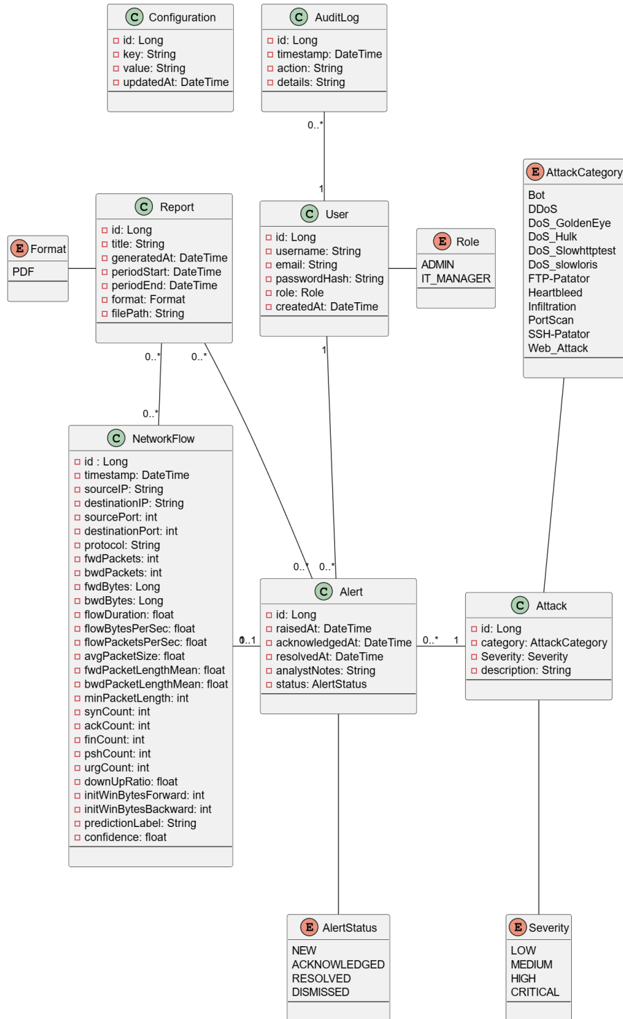
FIGURE 3.2 – Class Diagram
