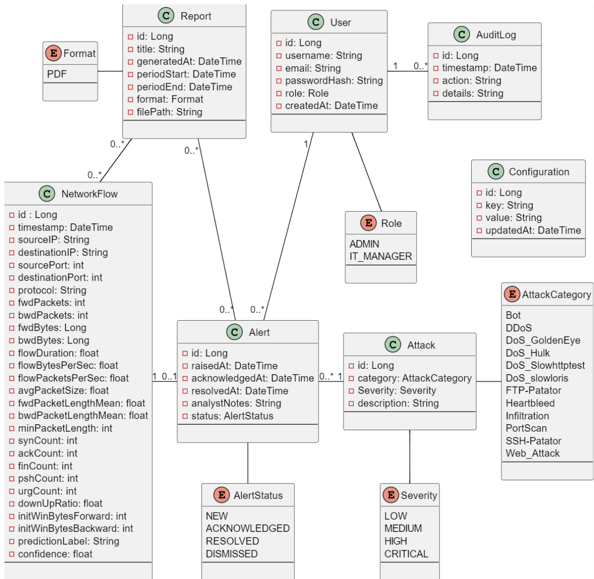
FIGURE 3.3 – Class Diagram
