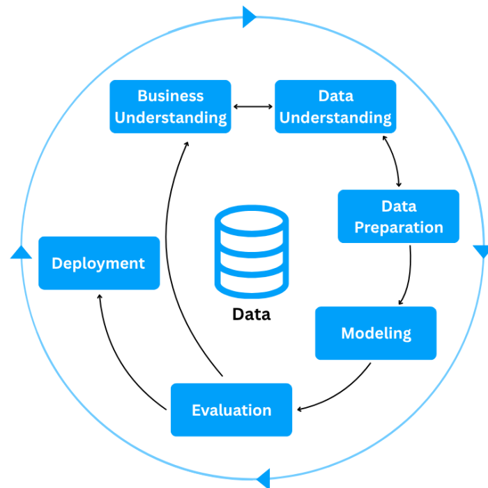
FIGURE 1.3 – CRISP-DM Methodology
