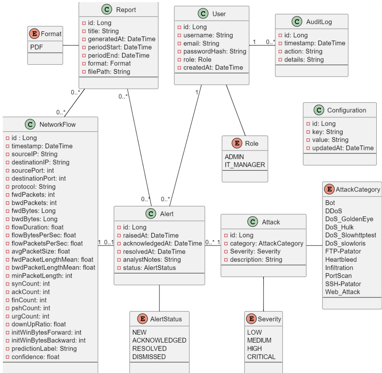
FIGURE 3.3 – Class Diagram
