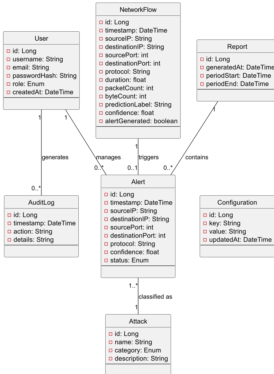
FIGURE 3.1 – Class Diagram
