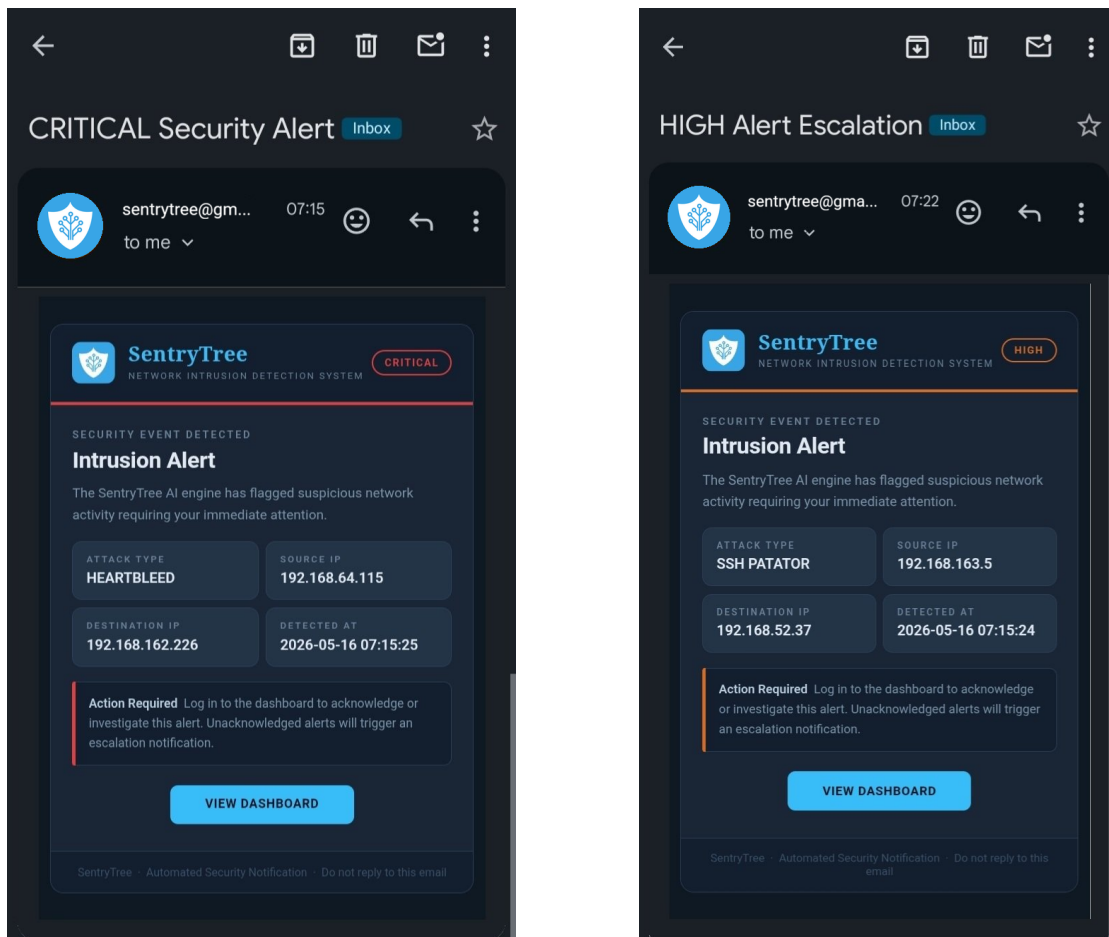
FIGURE 6.11 – Email notifications
