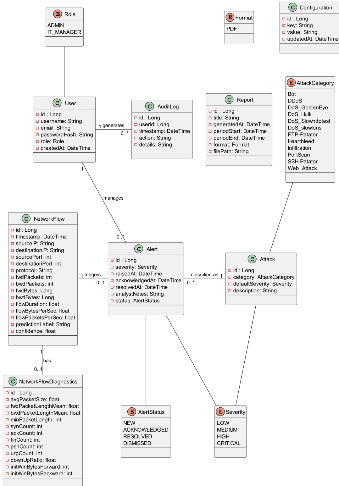
FIGURE 3.1 – Class Diagram
