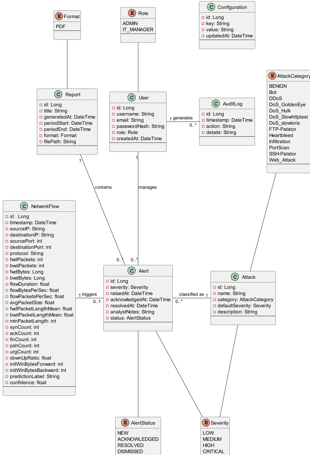
FIGURE 3.1 – Class Diagram
