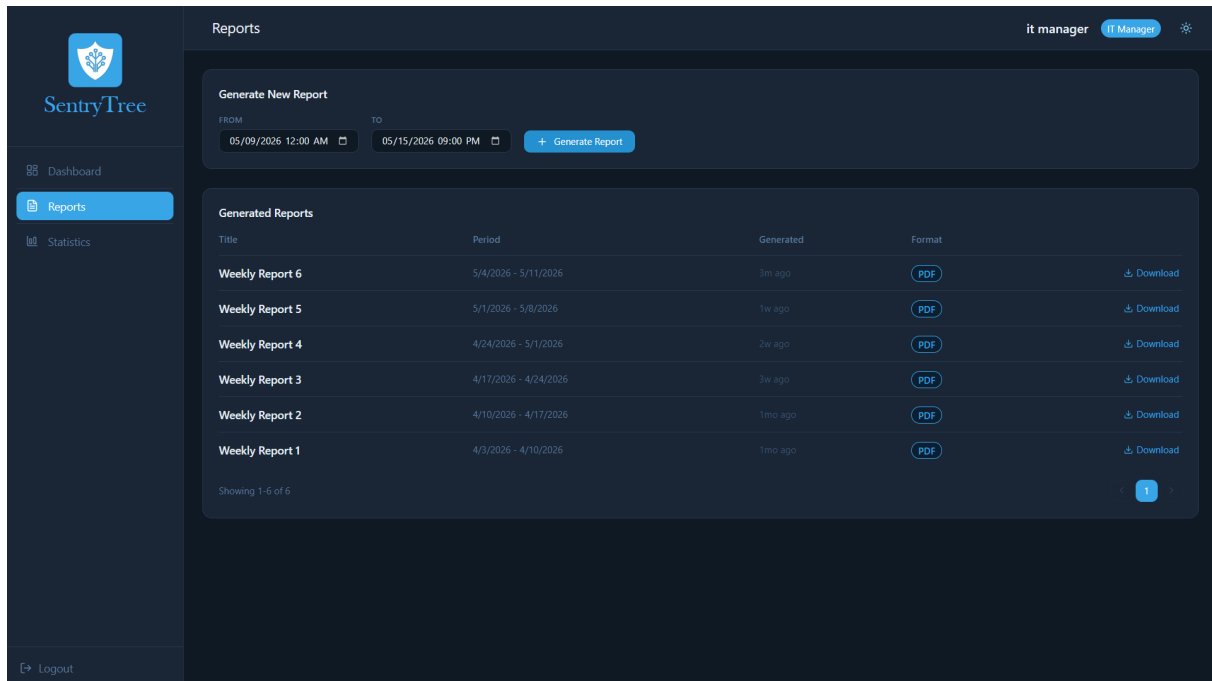
FIGURE 6.16 – Reports interface
