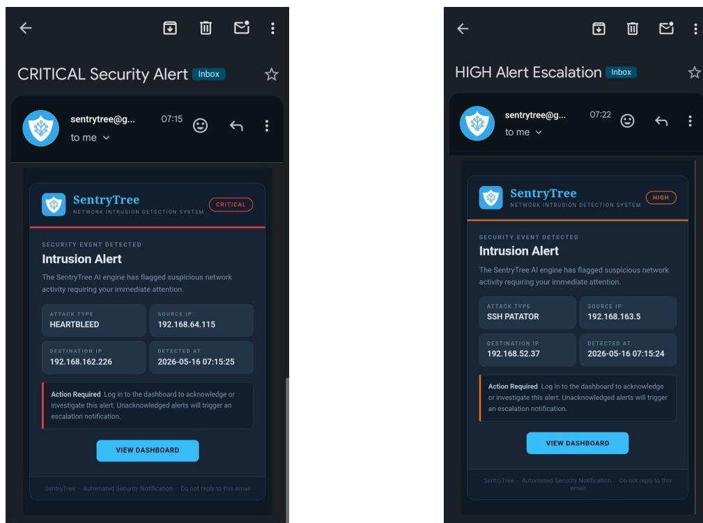
FIGURE 6.11 – Email notifications
