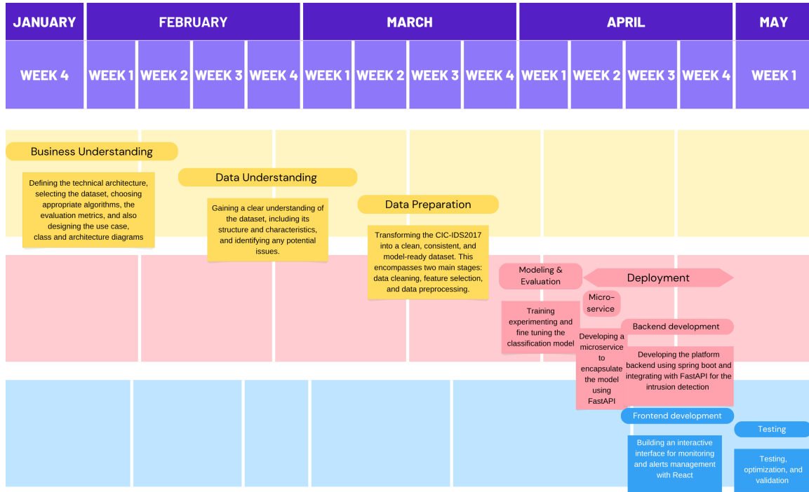
FIGURE 1.1 – Project Pipeline
