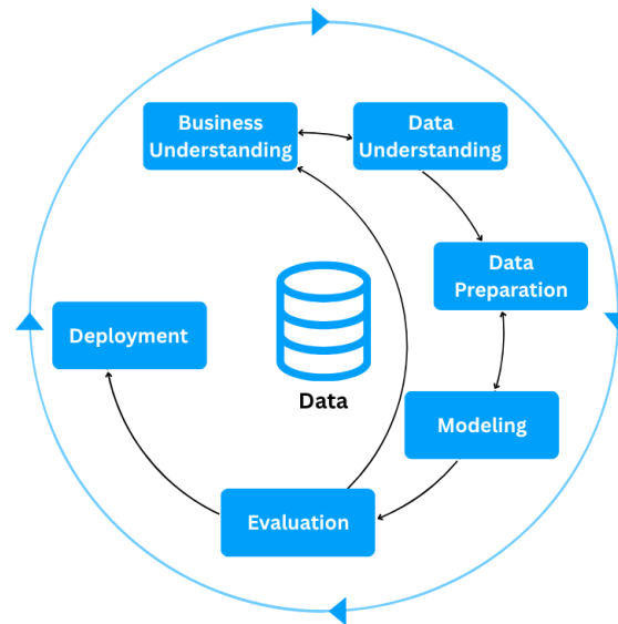
FIGURE 1.2 – CRISP-DM Methodology
