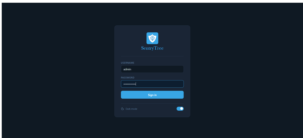
FIGURE 6.5 – Authentication interface
