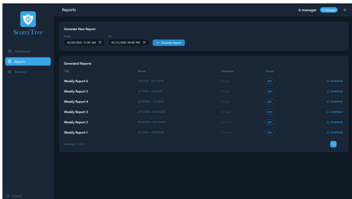
FIGURE 6.16 – Reports interface
