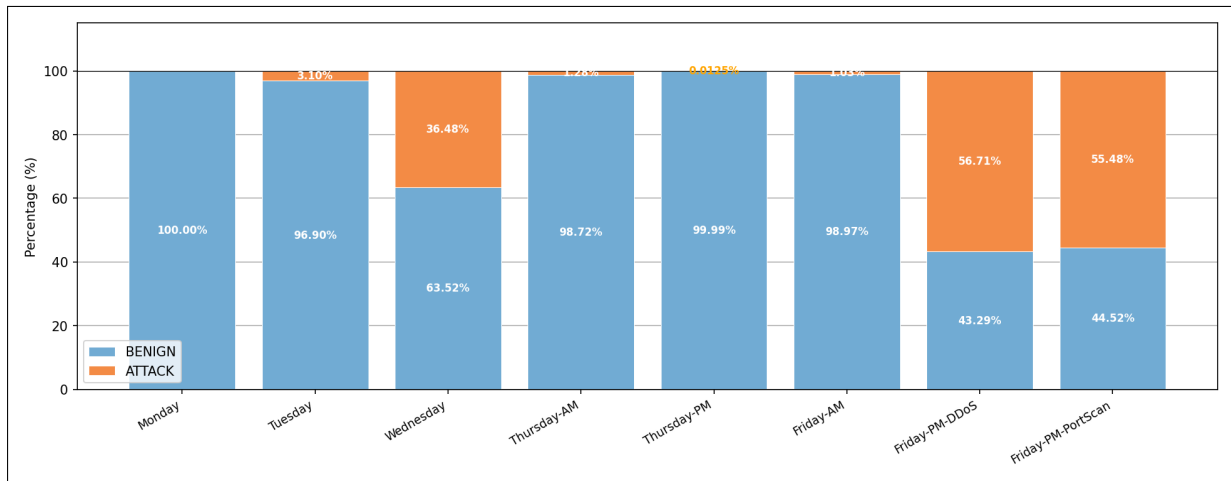
FIGURE 4.3 – Benign vs Attack Ratio per file
