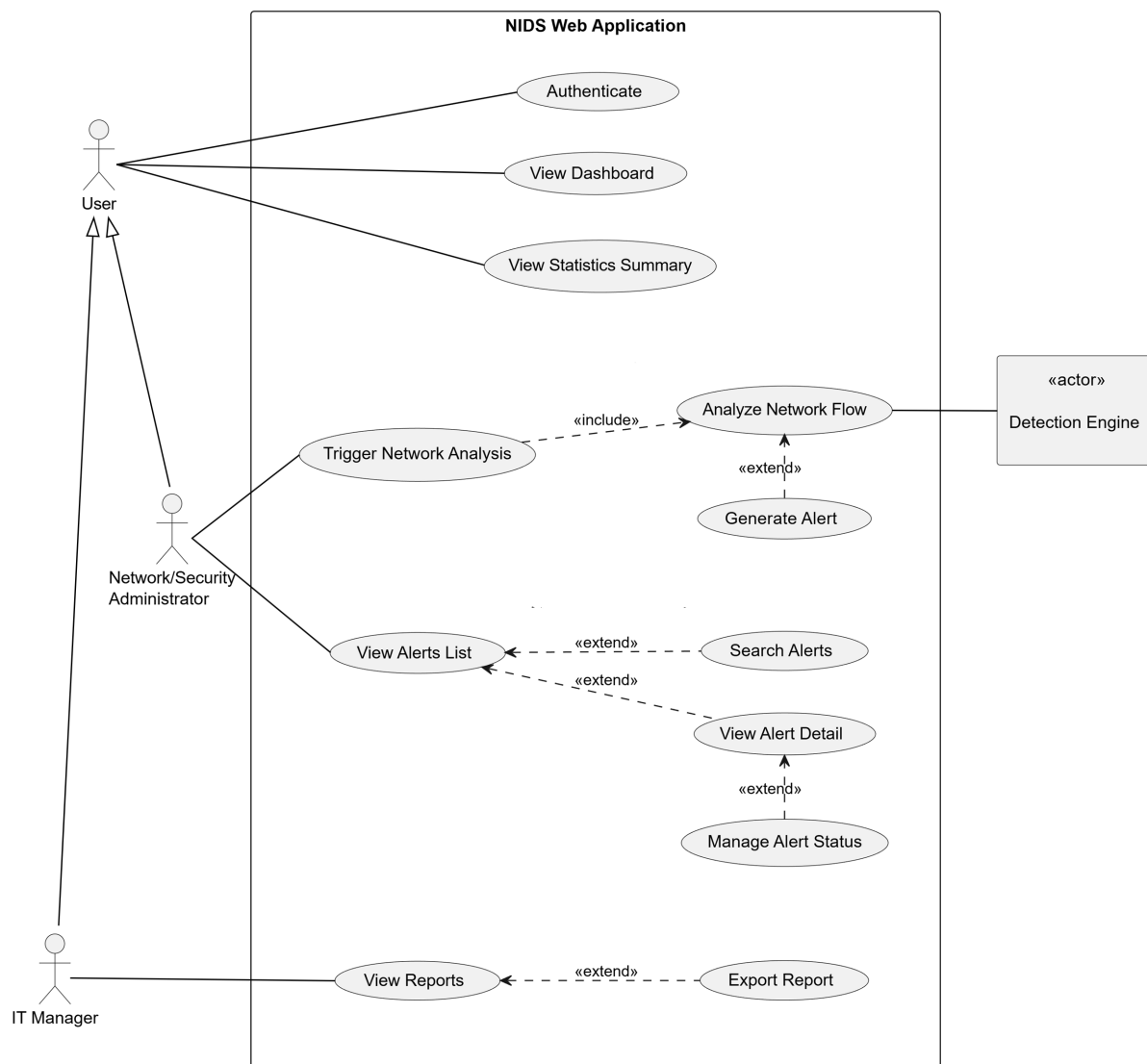
FIGURE 2.2 – Use Case Diagram
