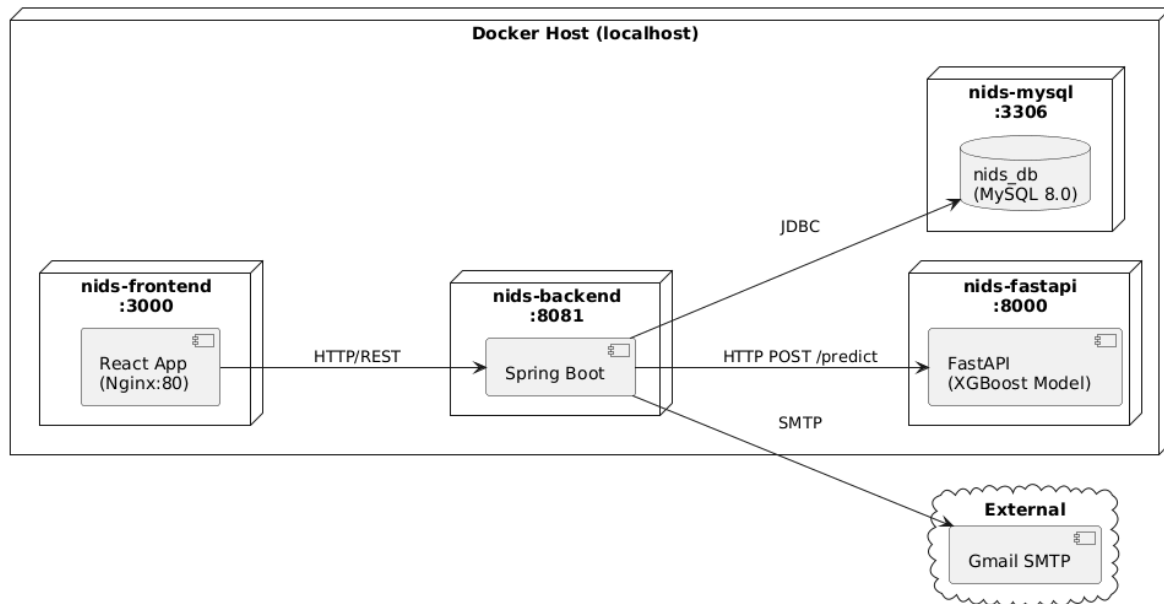
FIGURE 6.4 – Deployment Diagram
