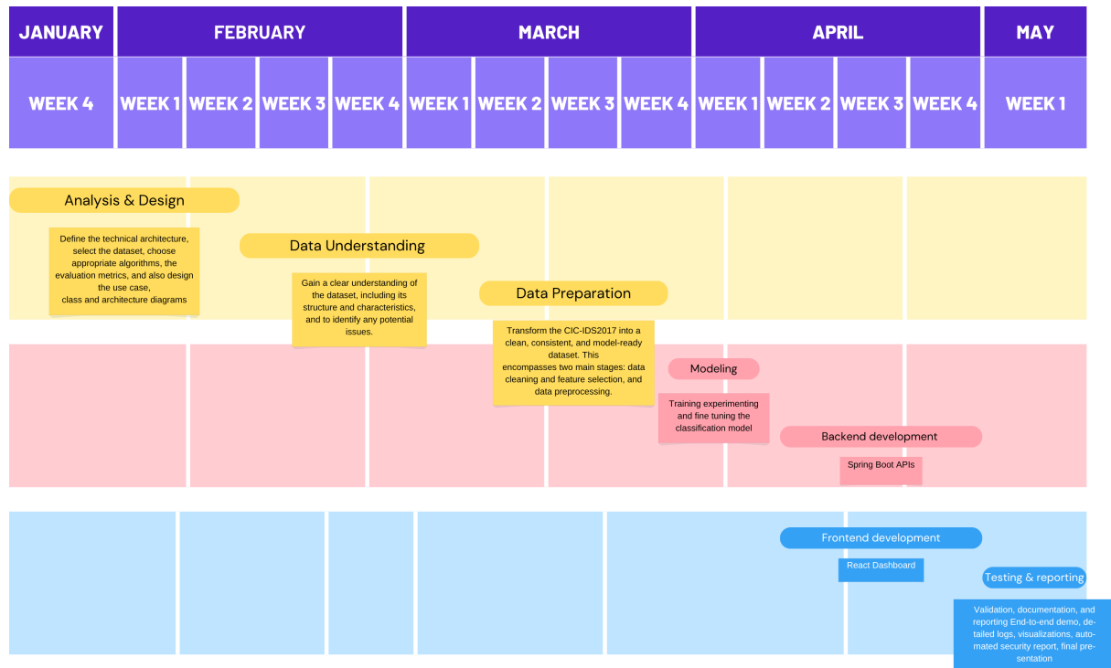
FIGURE 1.1 – Project pipeline
