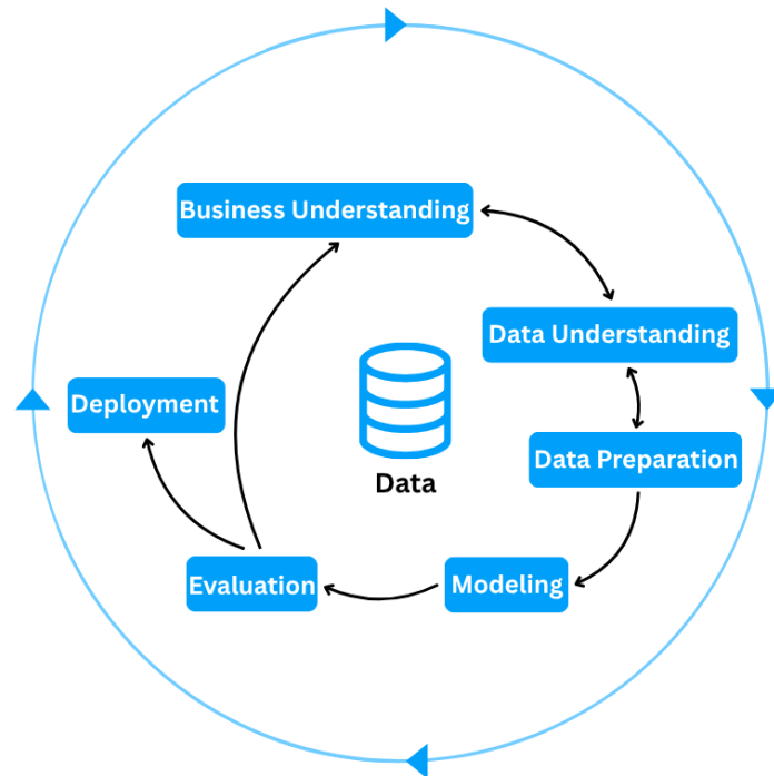
FIGURE 1.2 – CRISP-DM methodology
