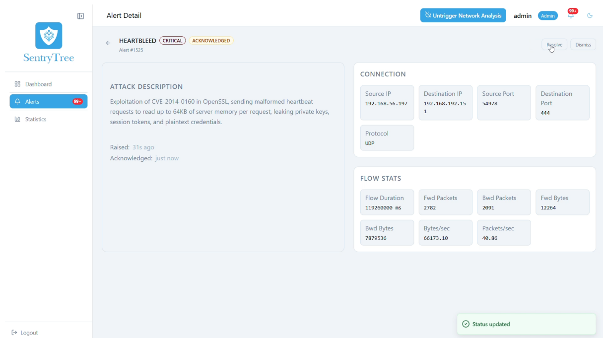
FIGURE 6.15 – Manage alert status interface
