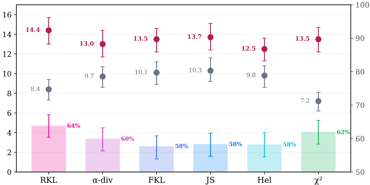
Arena-Hard win rate vs gpt-4-0314 (%)
