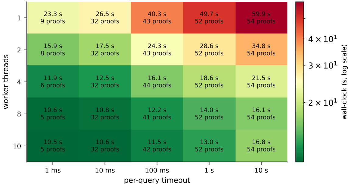
ODeSSy-stage wall-clock, zlib deflate.c (x86)
