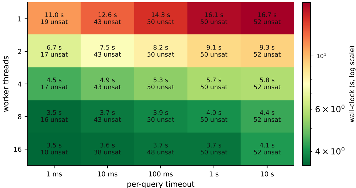
Oracle-stage wall-clock, zlib deflate (unsigned, O1)
