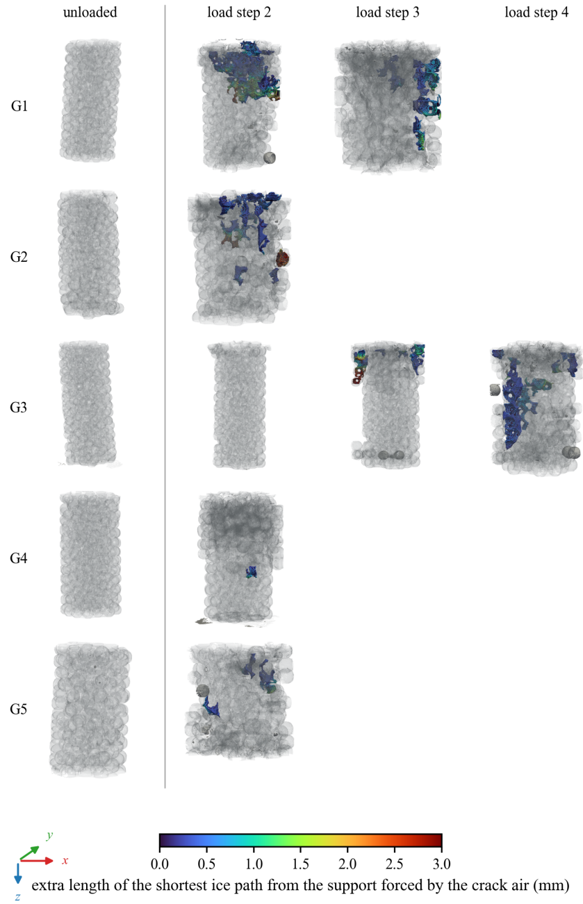
Figure S5: Ice-path maps of the glass specimens.
