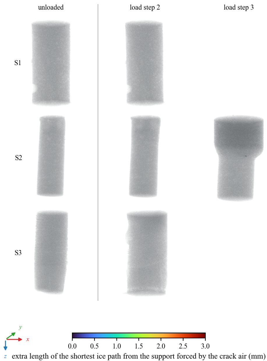
Figure S7: Ice-path maps of the sand specimens.
